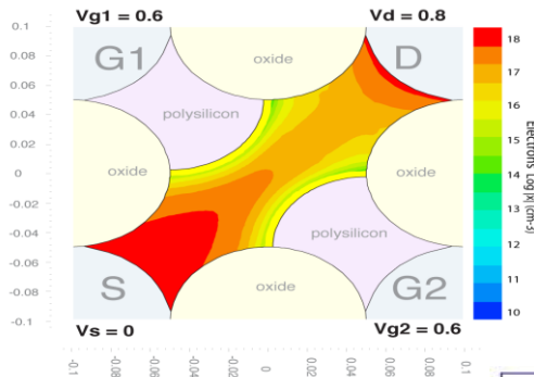
TCAD simulations
